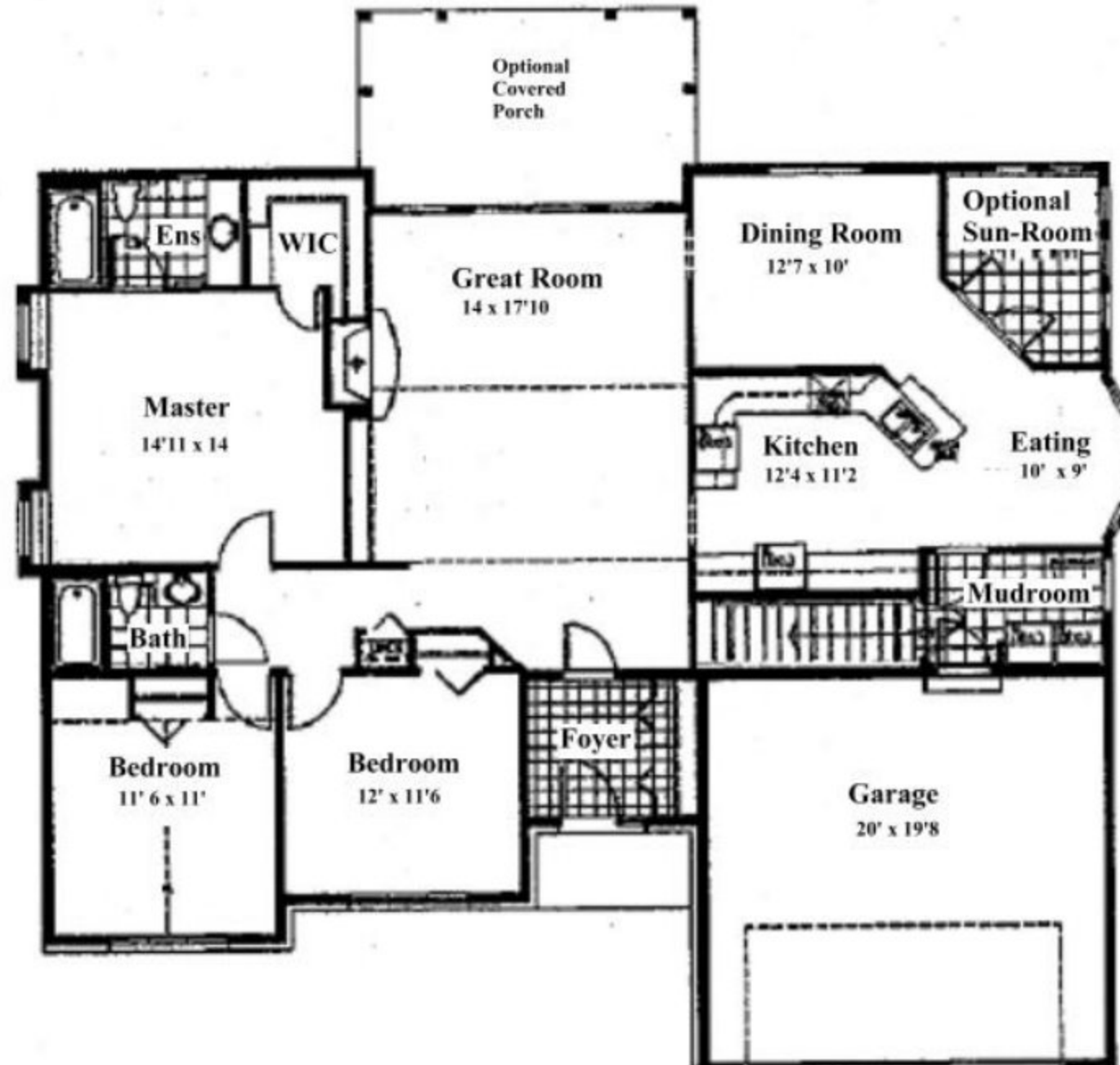
Ground Floor
